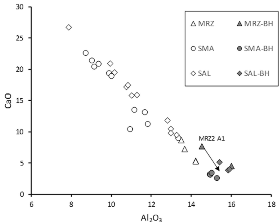
Fig. 5 \text{CaO} vs. \text{Al}_2\text{O}_3 diagram emphasizing the peculiarity of BHs. An arrow has been placed in correspondence with sample MRZ_2A1 to suggest that the pristine features of this horizon have been altered by the late precipitation of carbonate, as testified by field observations
